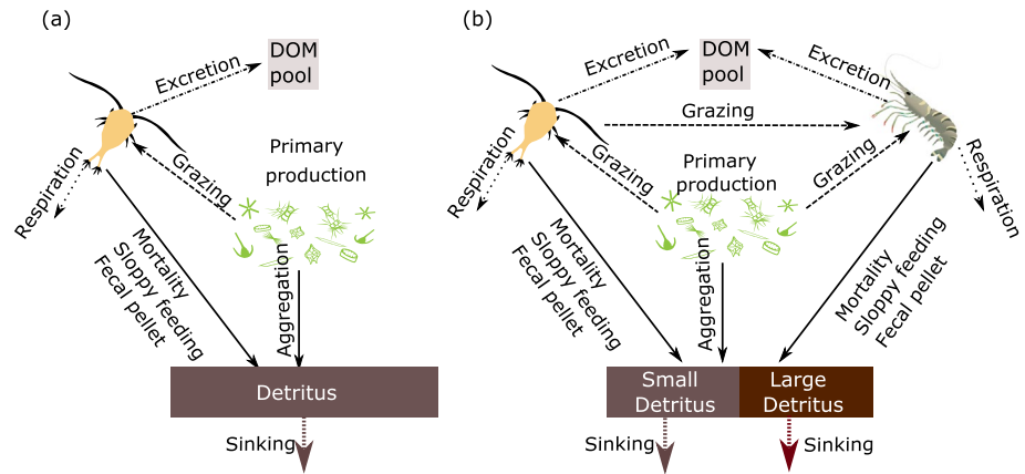
Figure 1. Processes in biogeochemistry model (a) REcoM-2, (b) REcoM-2-M with two zooplankton and a second, large detritus class. Both model versions represent primary production by two phytoplankton classes (nanophytoplankton and diatoms) and a small and fast-growing zooplankton group. In both versions, sinking detritus is produced via phytoplankton aggregation and through small zooplankton mortality, and a loss term accounting for sloppy feeding and fecal pellet production. Other loss processes for zooplankton biomass are respiration and excretion of dissolved organic matter. In addition, REcoM-2-M explicitly represents macrozooplankton with losses of sinking particulate organic matter being routed to a large detritus class with a higher sinking speed. The loss through fecal pellets is represented explicitly and macrozooplankton respiration varies in response to the seasonal cycle.
